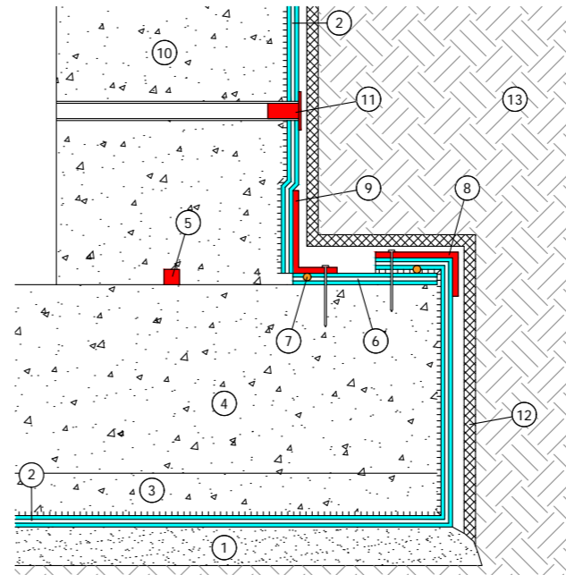
i1/i2/i3. Construction joint with Delta Amphibia pre-applied on formworks with toe
