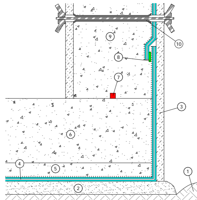
Construction joint with Delta Amphibia pre-applied on formworks without toe
