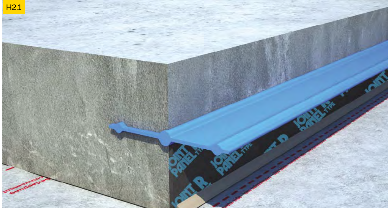
H2.1 RC raft foundation with Delta Amphibia - expansion joint with PVC waterstop
