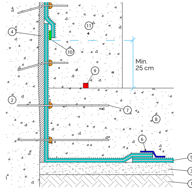
90° corner in case of blindside application with Delta Amphibia system
