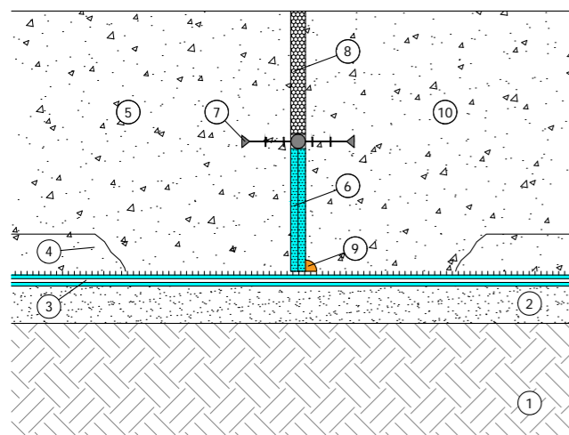
H2.1 RC raft foundation with Delta Amphibia - expansion joint with PVC waterstop
