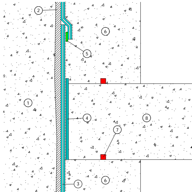
Application of hydro-expanding rubber joint panel type R for concrete slab sealing
