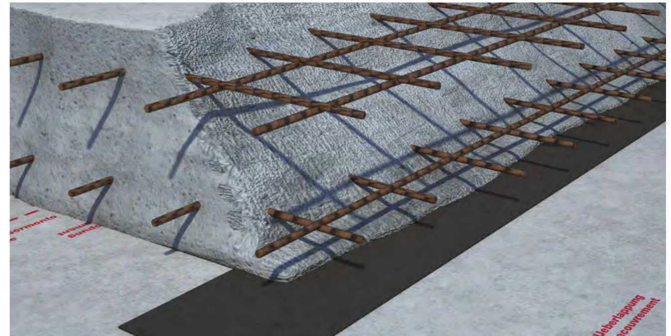
Detail of Delta Amphibia WT Waterstop Range
