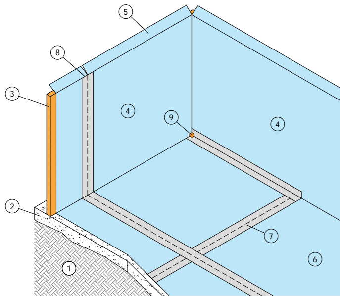
90° corner in case of open basement excavation with Delta Amphibia system
