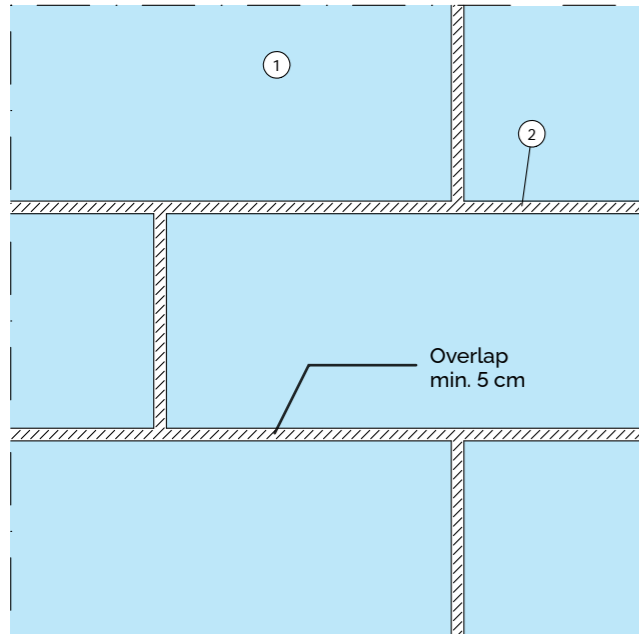
Raft foundation with Delta Amphibia system
