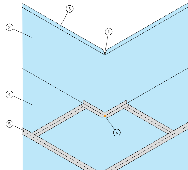
E1.1/E1.2/E1.3/E1.4/E1.5 Sealing of internal 90° corner on formworks
