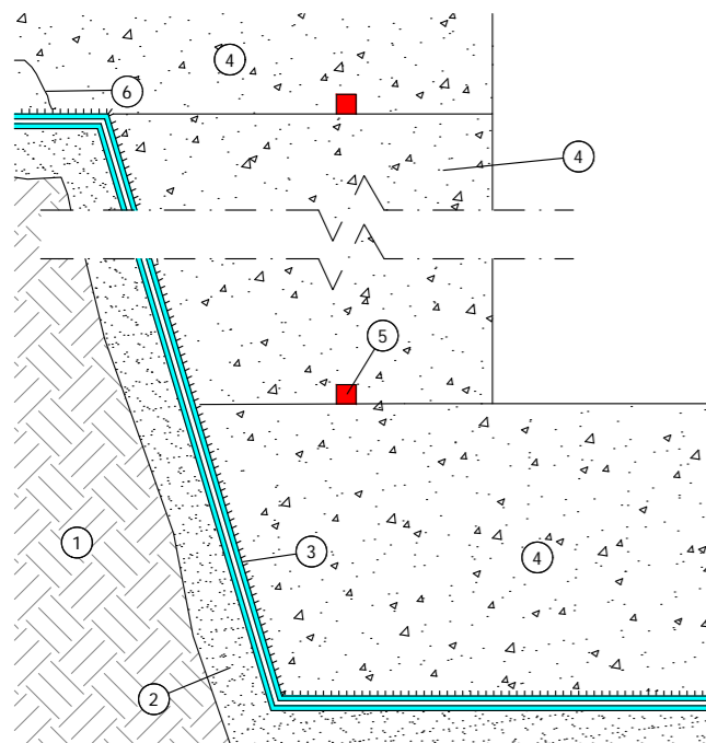
Lift pit with Delta Amphibia system
