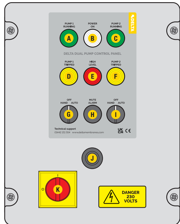
Delta Dual Pump Control Panel
